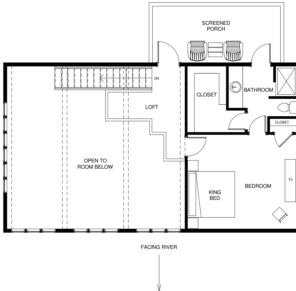
A EXISTING SECOND FLOOR PLAN Scale: 1/8" = 1'-0"
