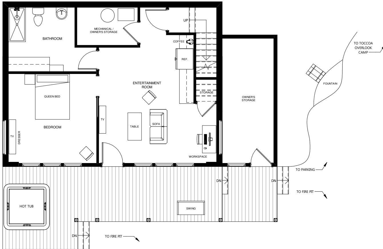
A LOWER LEVEL FLOOR PLAN Scale: 1/8" = 1'-0"
